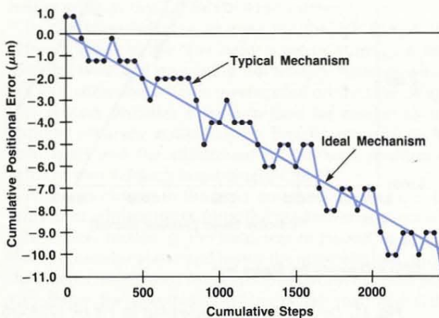
Fig. 8. Typical head positioning error plot for an HP 9145A Tape Drive.
