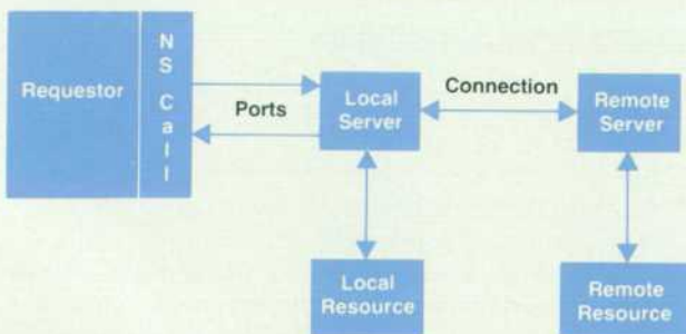
Fig. 10. The two-server model is used for virtual terminal and network file transfer services.
