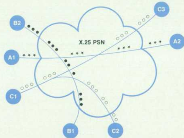
Fig. 3. X.25-based packet switched network virtual circuits.
