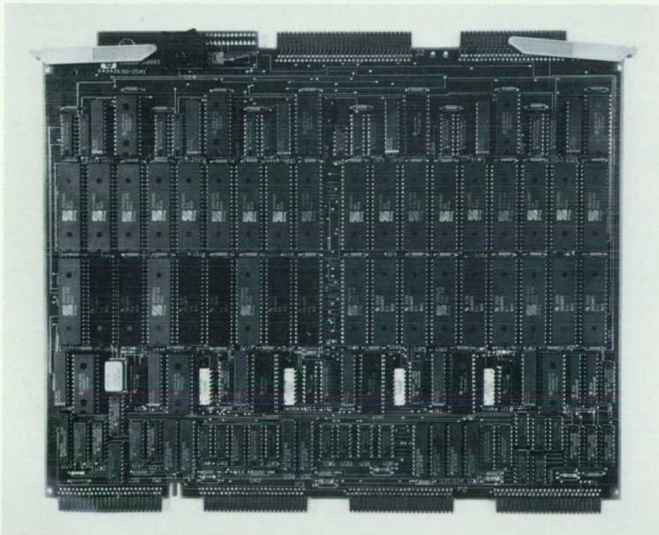
Fig. 5. MUX card.
