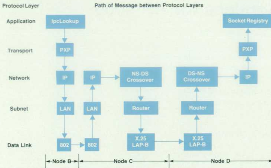
Fig. 6. Example 1 in the text describes the path of an IpcLookup request sent from node B to node D. This diagram summarizes which protocol layers are involved at each node.
