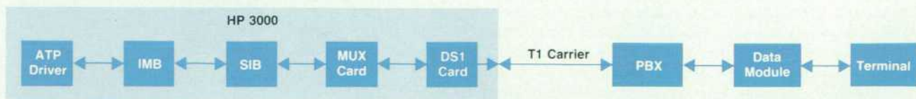
Fig. 2. DMI and HP 3000 components. (ATP=Advanced Terminal Processor, IMB=Inter-module Bus, SIB=System Interface Board.)
