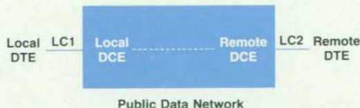
Fig. 7. X.25 procedures apply at the DTE/DCE interfaces.
