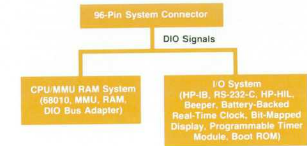
Fig. 1. Basic system partitioning of the Model 310 processor board.
