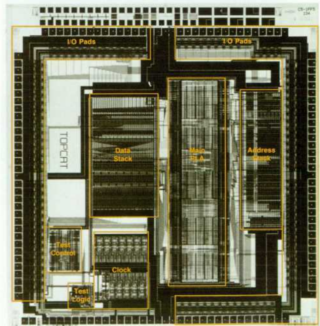
Fig. 2. Photograph of custom display controller chip.
