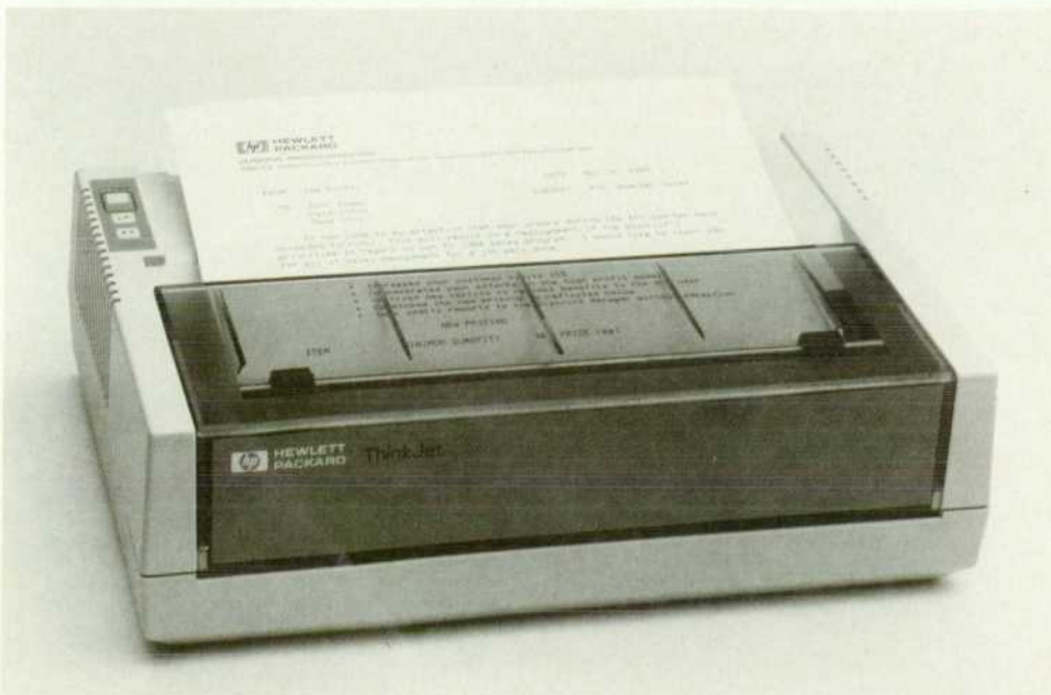
Fig. 1. The low-cost HP 2225 family of ThinkJet Printers provides fast, quiet, high-quality printing in a portable package. Four interface options and ac or battery operation are available.
