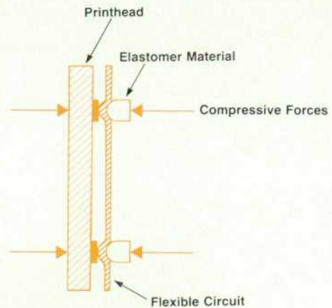
Fig. 2. The contact area of the flexible circuit is backed with an elastomer material and the whole assembly is compressed against the printhead contacts using a lever-activated cam. The elastomer provides a continuous force pushing the flexible circuit dimples against the mating printhead pads.
