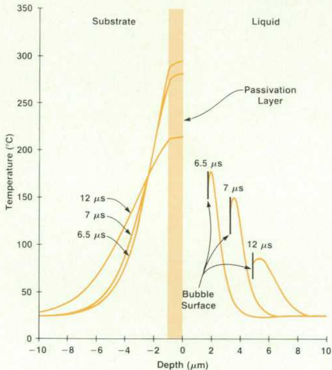
Fig. 6. Temperature profiles after bubble nucleation at 6 \mu\text{s} calculated from one-dimensional model. The bubble forms on top of the passivation layer and grows to the right.
