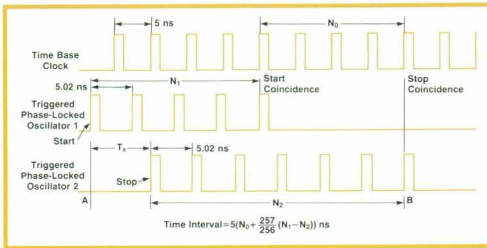
Fig. 2. Dual vernier method interpolates within the 5-ns period of the 5370A's 200-MHz time-base clock to obtain 20-ps resolution. The start and stop pulses start the oscillations of two triggered phase-locked oscillators. Coincidences of the oscillator waveforms with the time base clock define the counts N_0 , N_1 , and N_2 , as shown. The unknown time interval is computed from these counts.
