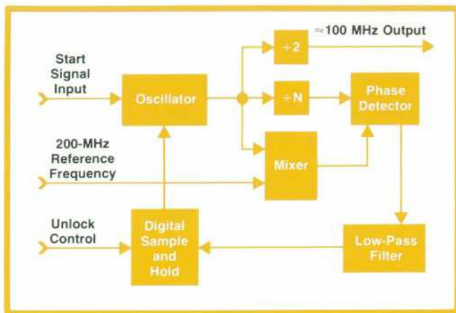
Fig. 6. A triggered phase-locked oscillator generates the clock frequency counted by the digital delay circuits. A sample-and-hold circuit is activated when the selected (width + delay) is short. The circuit measures the VCO voltage during phase-locked conditions and holds that value during high-repetition rate operation.
