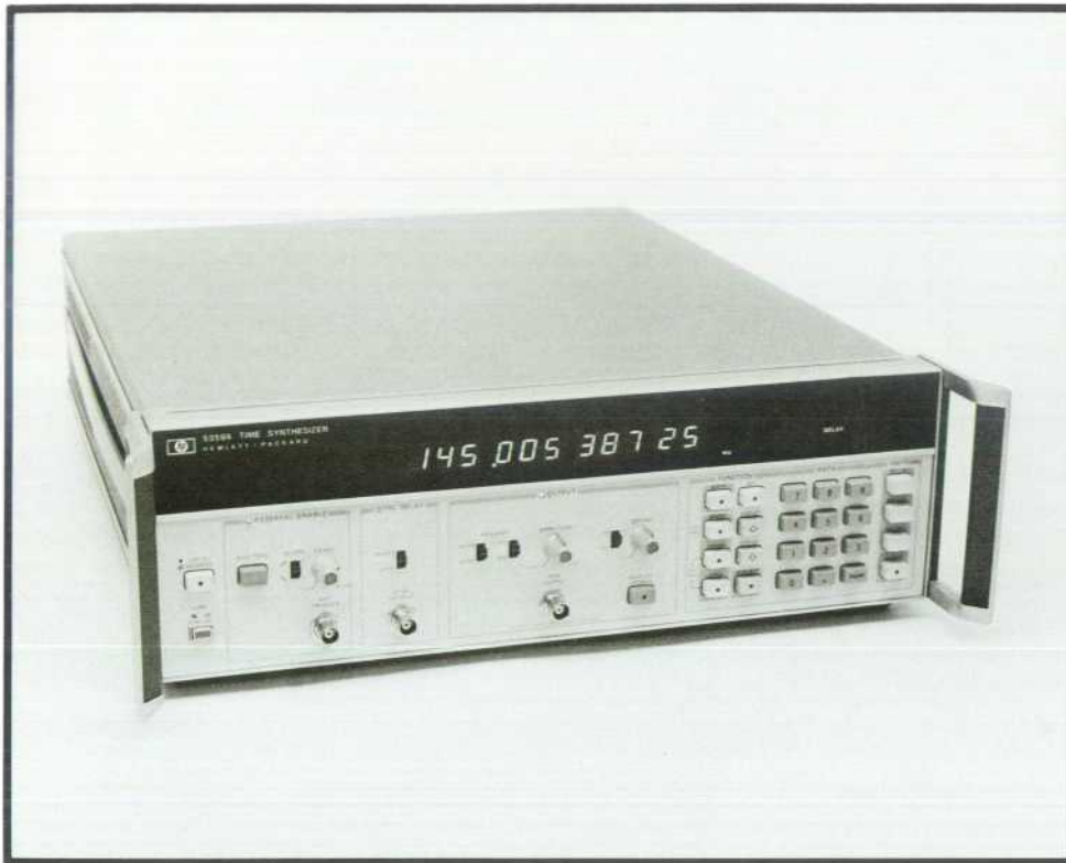
Fig. 2. Model 5359A Time Synthesizer generates precise time delays and pulse widths from 0 to 160 ms (width + delay \leq 160 ms). Absolute accuracy is \pm 1 ns \pm time base error. With the optional high-stability time base, jitter is < 200 ps rms (100 ps typical). Features include keyboard control, HP-IB programmability, and automatic calibration.
