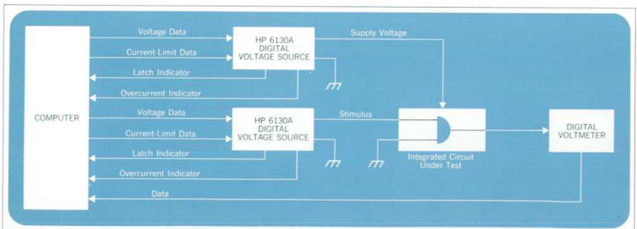
Fig. 1. Semiconductor Testing
