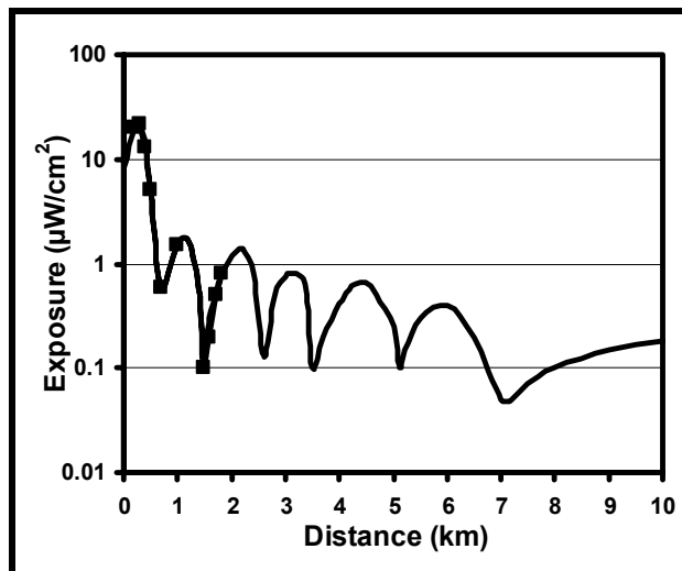
Figure 32: The measured and estimated power density (exposure in \mu\text{W}/\text{cm}^2 ) with distance from the Sutra Tower. Squares show the 1988 measurements. The line follows measurement points and the radial pattern of a typical UHF transmission beyond 2 km. From Hammett and Edison (1997).
