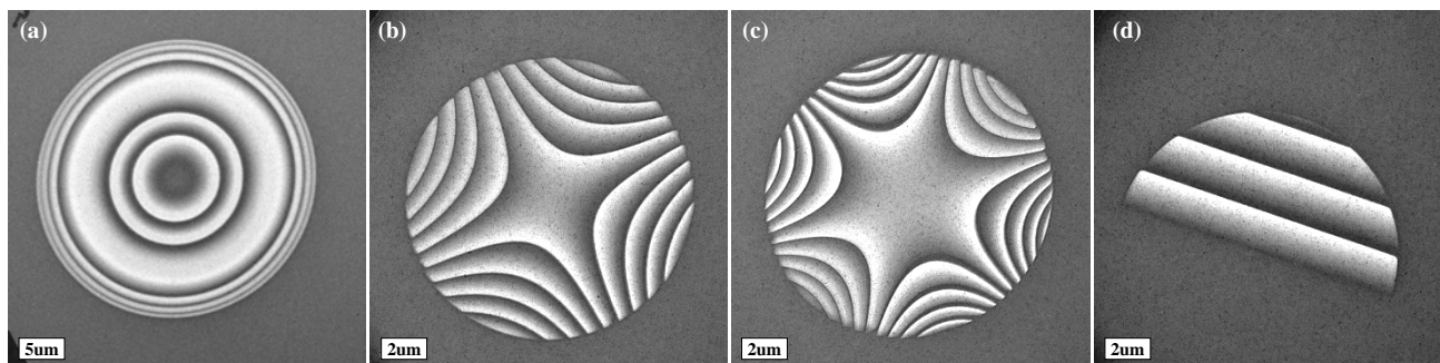
Figure 1. TEM images of phase-masks imparting (a) spherical, (b) astigmatic, (c) trefoil, and (c) half-beam tilt phase to the electron-beam. Contrast and brightness have been changed for visibility.
