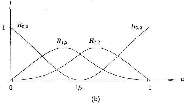
Figure 7.20. Semicircle of Figure 7.15 after inserting u = 1/2 one time. (a) Control polygon and parameterization; (b) rational basis functions.
