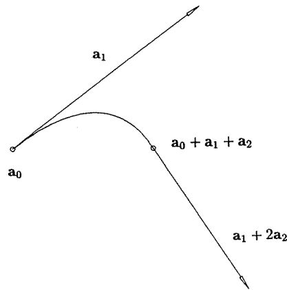
Figure 1.6. Parabolic arc, C(u) = a_0 + a_1u + a_2u^2 .
