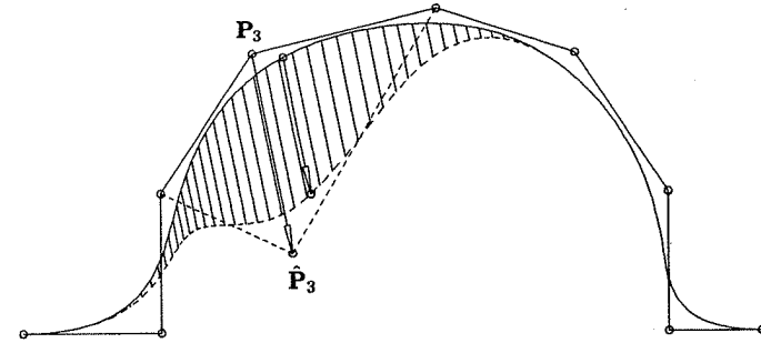
Figure 11.2. Moving \mathbf{P} = \mathbf{C}(\bar{u} = 0.37) by repositioning \mathbf{P}_3 ; the corresponding node is t_3 = 0.35 , and the curve degree is three. Notice the parallel translation of a segment of the curve.
