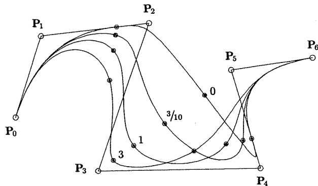
Figure 4.2. Rational cubic B-spline curves, with w_3 varying.
