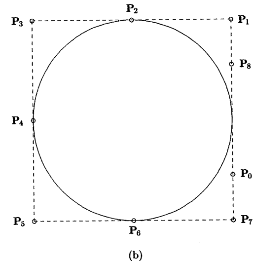
Figure 12.5. Unclamping the nine-point NURBS circle. (a) Original curve; (b) unclamped curve.
