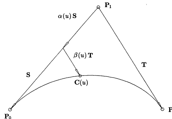
Figure 7.11. Local coordinate system for rational quadratic Bézier curve.
