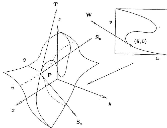
Figure 6.4. Surface tangent vector inversion.
