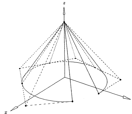
Figure 8.6. A right circular conical patch.
