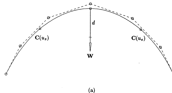
Figure 11.19. Curve warping. (a) The original curve with span [\mathbf{C}(u_s), \mathbf{C}(u_e)] to be warped in the direction of \mathbf{W} a distance d ; (b) a curve span refined; (c) control points repositioned; (d) knots removed.
