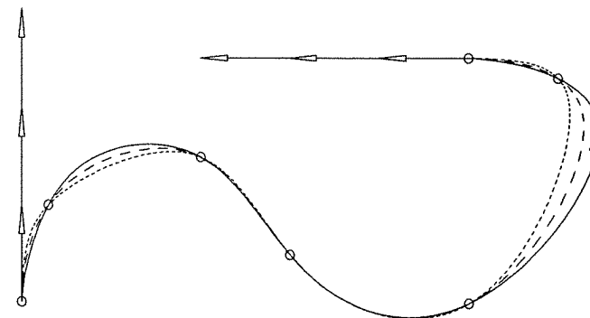
Figure 9.8. Global cubic curve interpolants with varying end derivative magnitudes.
