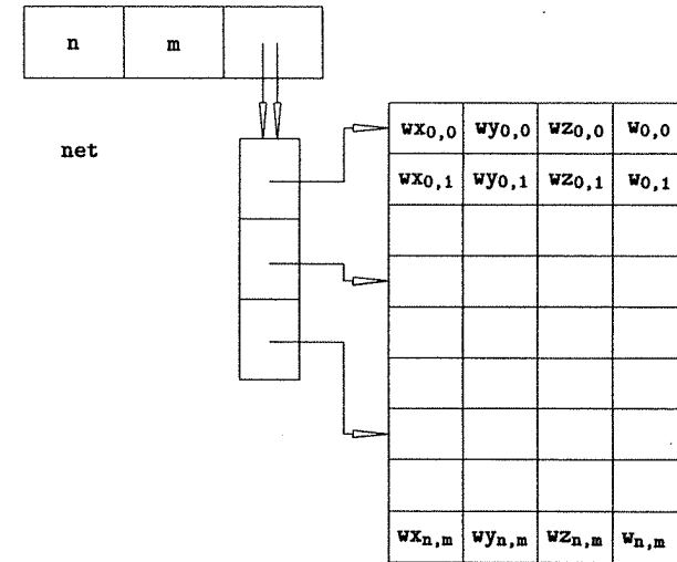
Figure 13.5. Control net data structure.
