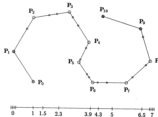
Figure 5.4. Nonuniform partitioning of the control polygon in Figure 5.3a defined by the knot vector \{0, 0, 0, 0, 1, 1.5, 2.3, 3.9, 4.3, 5, 6.5, 7, 7, 7\} .
