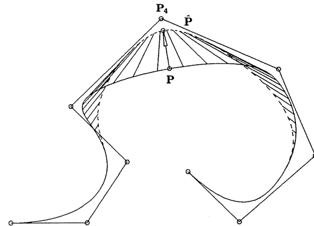
Figure 11.11. Pulling the curve at t_4 = u = 0.52 a distance d = 0.075 toward \mathbf{P}_4 by changing the weight w_4 = 0.2 ; the new weight computed is \hat{w}_4 = 2.45 . Notice the perspective translation of the curve segment produced by the change of weight.
