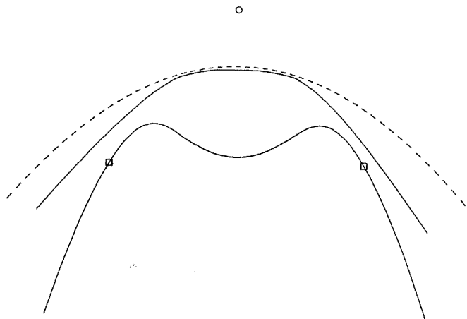
Figure 11.31. Parabolic bending used to eliminate inflexion points.
