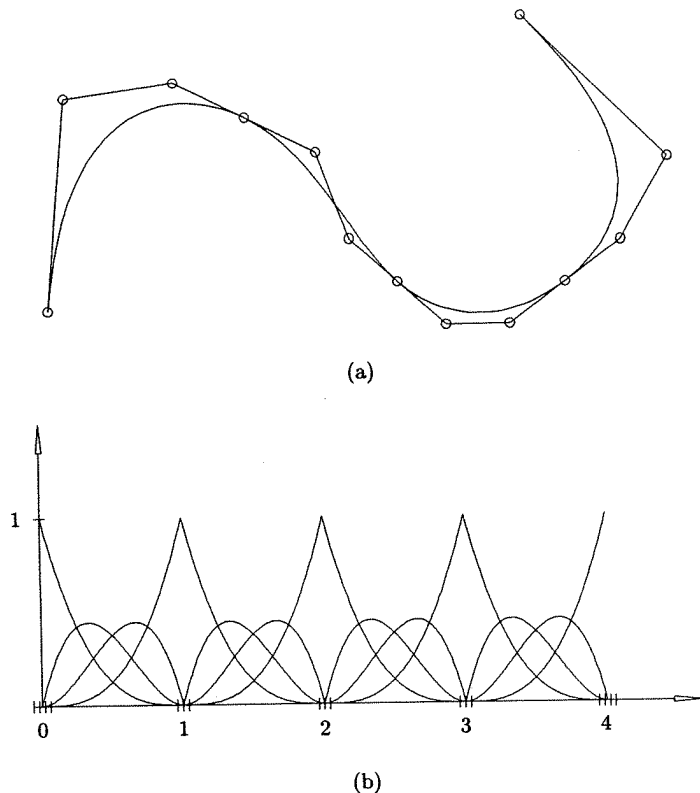
Figure 5.19. Decomposition of the curve in Figure 5.18 into a piecewise Bézier curve via knot refinement. (a) The decomposed curve and its control polygon; (b) basis functions after inserting knots 1, 2, and 3 two times each.
