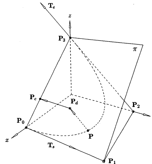
Figure 9.55. A unique cubic three-dimensional (twisted) Bézier curve specified by endpoints, end tangents, and one point on the curve.
