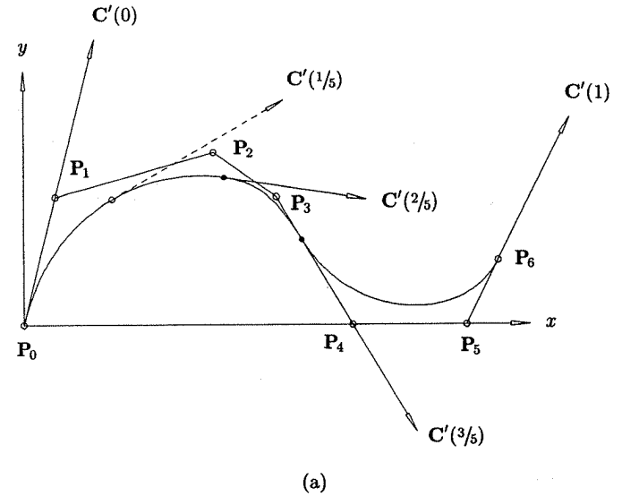
Figure 3.16. (a) A cubic curve on U = \{0, 0, 0, 0, 2/5, 3/5, 3/5, 1, 1, 1, 1\} ; (b) the quadratic derivative curve on U' = \{0, 0, 0, 2/5, 3/5, 3/5, 1, 1, 1\} .
