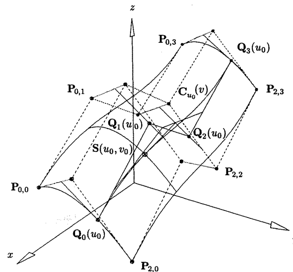
Figure 1.25. The deCasteljau algorithm for a Bézier surface.
