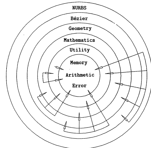
Figure 13.9. Nlib V2.0 's system structure.
