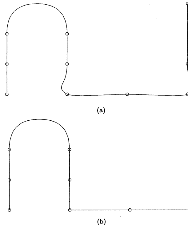
Figure 9.24. Local quadratic curve interpolants. (a) No corner is allowed; (b) the corner is maintained.
