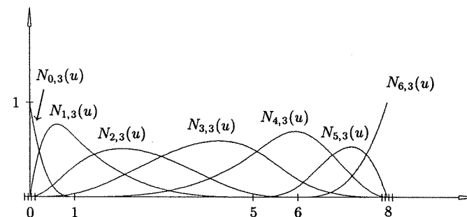
Figure 2.12. Nonuniform cubic basis functions defined on U = \{0, 0, 0, 0, 1, 5, 6, 8, 8, 8, 8\} .
