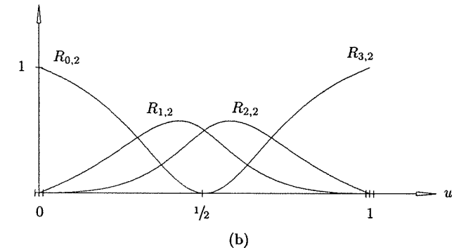
Figure 7.19. Arc of Figure 7.18 after inserting u = 1/2 one time. (a) Control polygon and parameterization; (b) rational basis functions.
