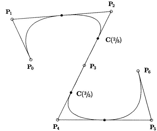
Figure 3.6. A quadratic B-spline curve on U = \{0, 0, 0, 1/5, 2/5, 3/5, 4/5, 1, 1, 1\} . The curve is a straight line between C(2/5) and C(3/5) .
