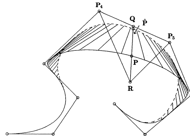
Figure 11.15. Simultaneous pull at u = 1/2(t_4 + t_5) = 0.608 a distance d = 0.088 in the direction of \mathbf{R}\mathbf{Q} by changing w_4 = w_5 = 0.05 ; the new weights are \hat{w}_4 = \hat{w}_5 = 1.23 . The curve change is neither perspective nor parallel.
