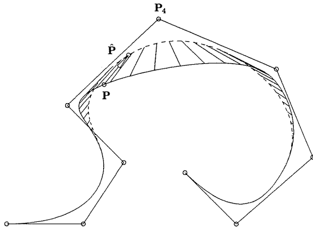
Figure 11.12. Pulling the curve at u = 0.46 a distance d = 0.075 toward P_4 by changing the weight w_4 = 0.2 ; the new weight computed is \hat{w}_4 = 0.97 .
