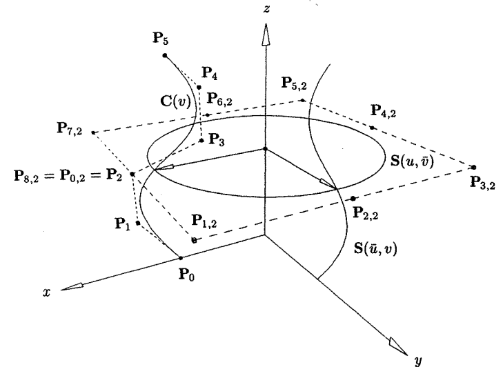
Figure 8.8. Definition of a surface of revolution.
