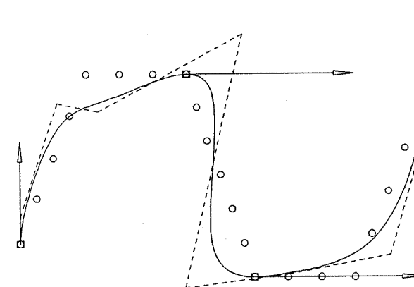
Figure 9.42. The curve from Figure 9.40, but using two new tangent constraints.
