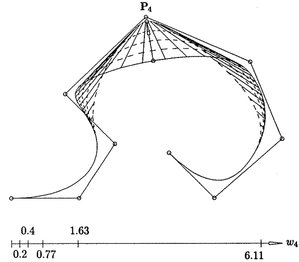
Figure 11.13. Pulling the curve at t_4 = u = 0.52 with equal increments \Delta = 0.022 toward P_4 by changing the weight w_4 = 0.2 ; the new weights computed are \hat{w}_4 = \{0.4, 0.77, 1.63, 6.11\} .
