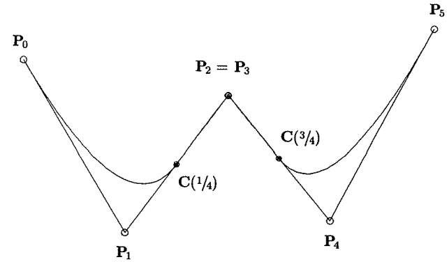
Figure 3.13. A quadratic curve on U = \{0, 0, 0, 1/4, 1/2, 3/4, 1, 1, 1\} ; P_2 = P_3 is a double control point.
