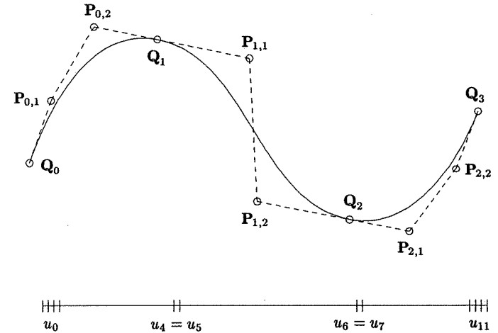
Figure 9.29. C^1 local cubic curve interpolant.
