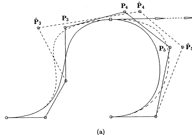
Figure 11.36. Constraint-based curve modification using positional and derivative constraints. (a) Derivative constraints are applied and P_3, P_4 , and P_5 are allowed to move; (b) derivative constraints are applied and only P_4 is allowed to move; (c) derivative and positional constraints are applied, and P_3 and P_4 are allowed to move.
