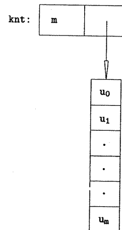
Figure 13.3. Knot vector data structure.
