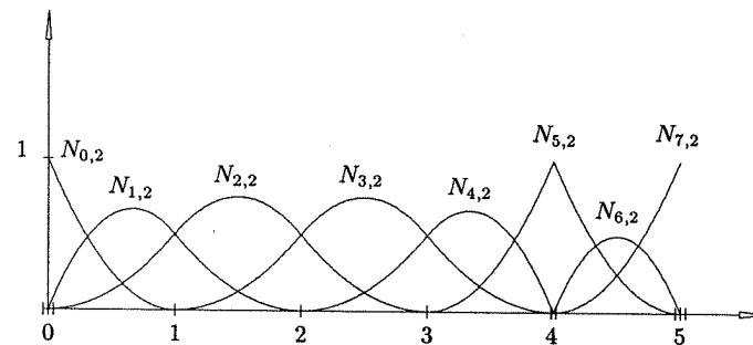
Figure 2.6. The nonzero second-degree basis functions, U = \{0, 0, 0, 1, 2, 3, 4, 4, 5, 5, 5\} .
