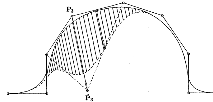
Figure 11.3. Moving \mathbf{P} = \mathbf{C}(\bar{u}) by repositioning \mathbf{P}_3 . \bar{u} = 0.43 = 1/2(t_3 + t_4) ; the corresponding node is t_3 = 0.35 , and the curve degree is three.
