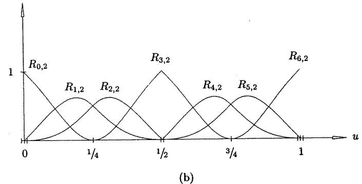
Figure 7.21. A seven-point square-based NURBS circle. (a) Control polygon and parameterization; (b) rational basis functions.
