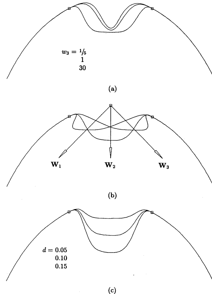
Figure 11.20. Curve warps (a) using different weights w_3 = \{1/5, 1, 30\} ; (b) using different directions with w_3 = 20 ; (c) using different distances d = \{0.05, 0.1, 0.15\} .
