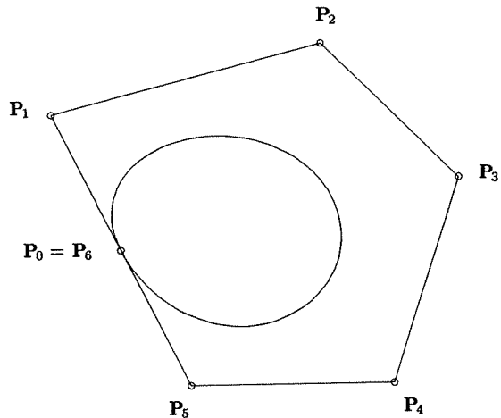
Figure 1.12. A smooth, closed, sixth-degree Bézier curve.
