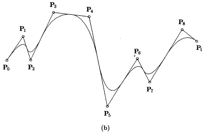
Figure 3.8. B-spline curves. (a) A ninth-degree Bézier curve on the knot vector U = \{0, 0, 0, 0, 0, 0, 0, 0, 0, 1, 1, 1, 1, 1, 1, 1, 1\} ; (b) a quadratic curve using the same control polygon defined on U = \{0, 0, 0, 1/8, 2/8, 3/8, 4/8, 5/8, 6/8, 7/8, 1, 1, 1\} .
