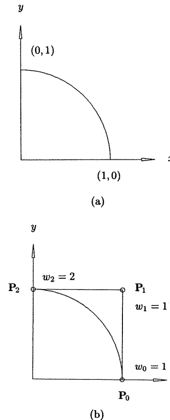
Figure 1.19. Representation of the unit circle. (a) x(u) = (1-u^2)/(1+u^2) and y(u) = (2u)/(1+u^2) for one quadrant; (b) the Bézier representation corresponding to Figure 1.19a ( w_0 = 1, w_1 = 1, w_2 = 2 ).
