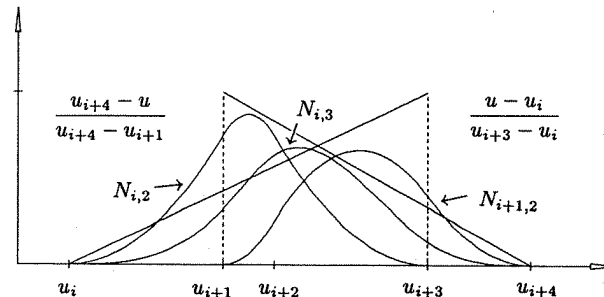
Figure 2.3. The recursive definition of B-spline basis functions.
