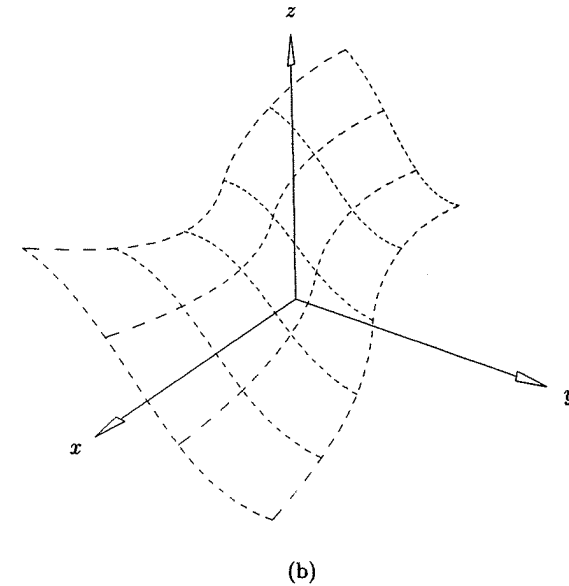
Figure 5.30. A (cubic \times quadratic) surface for knot removal. (a) The control net; (b) the surface defined over U = \{0, 0, 0, 0, 0.22, 0.3, 0.52, 0.7, 0.79, 1, 1, 1, 1\} and V = \{0, 0, 0, 0.2, 0.42, 0.5, 0.81, 0.9, 1, 1, 1\} .
