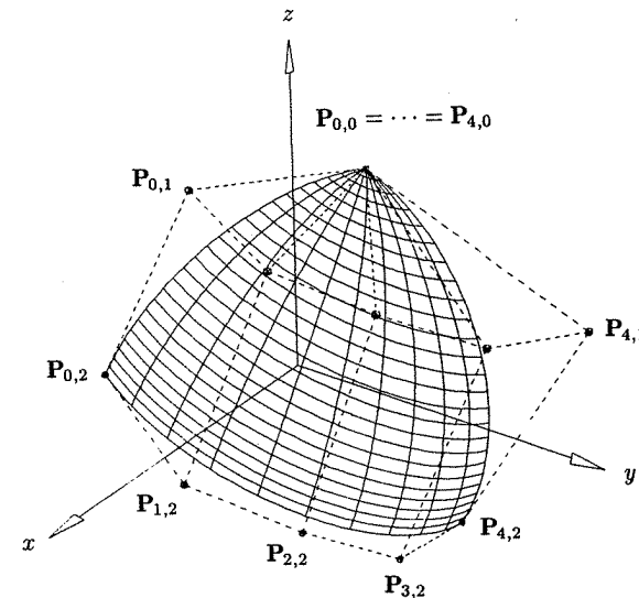
Figure 8.19. A corner fillet surface – an arbitrary spherical patch whose boundaries are great circles of the sphere.
