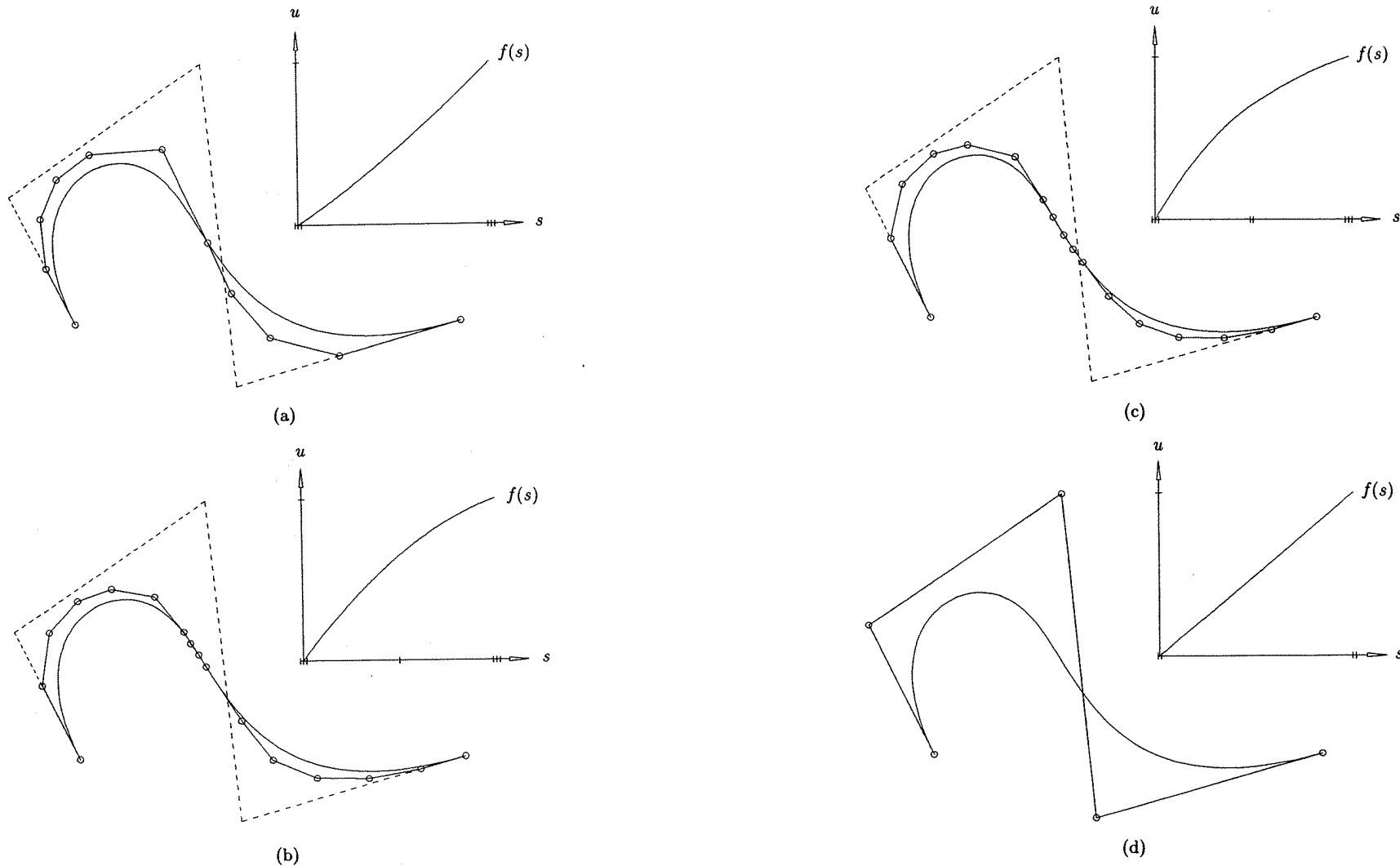
Figure 6.11. B-spline curve reparameterized with quadratic B-spline functions. (a) F = \{0, 2/5, 1\} , S = \{0, 0, 0, 1, 1, 1\} ; (b) F = \{0, 2/5, 9/10, 1\} , S = \{0, 0, 0, 1/2, 1, 1, 1\} .
