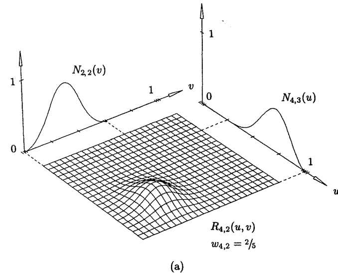
Figure 4.10. The basis function R_{4,2}(u,v) , with U = \{0, 0, 0, 0, 1/4, 1/2, 3/4, 1, 1, 1, 1\} and V = \{0, 0, 0, 1/5, 2/5, 3/5, 3/5, 4/5, 1, 1, 1, 1\} . w_{i,j} = 1 for all (i,j) \neq (4,2) . (a) w_{4,2} = 2/5 ; (b) w_{4,2} = 6 .
