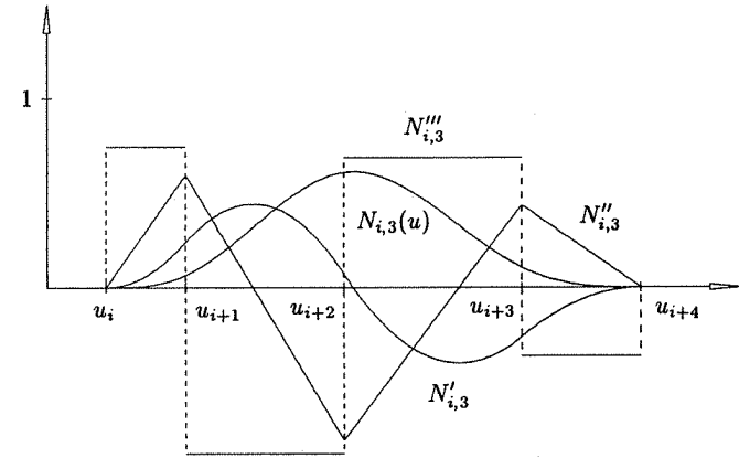
Figure 2.11. N_{i,3} and all its nonzero derivatives.
