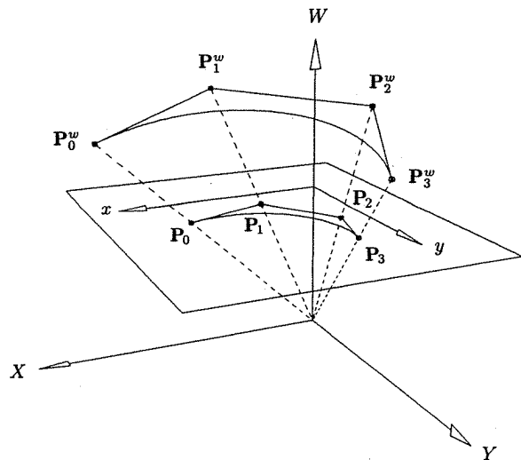
Figure 1.21. A geometric construction of a rational Bézier curve.
