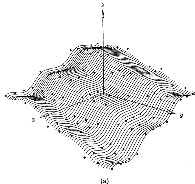
Figure 9.46. A least squares surface fit with a degree (2,3) surface using an (8×8) control net. (a) Surface approximant; (b) error surface (error measured at data points).
