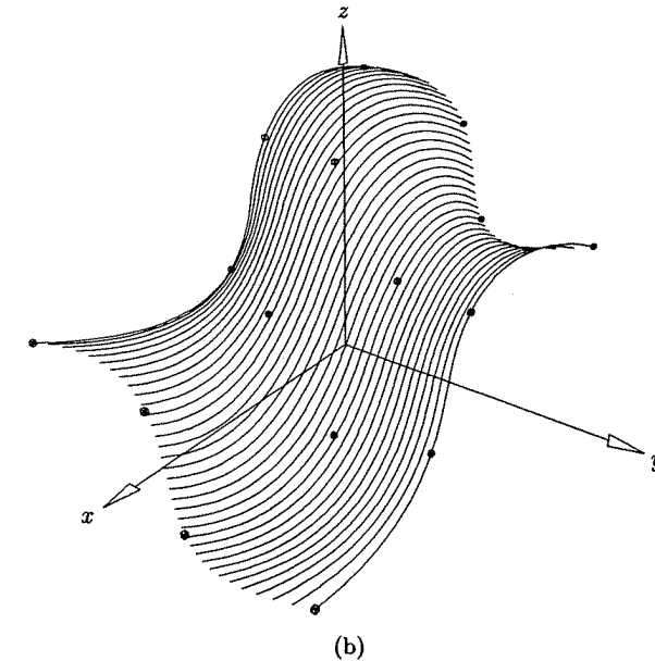
Figure 9.17. Surface interpolants using different degrees; the parameterization is chord length and knot vector obtained by averaging.
