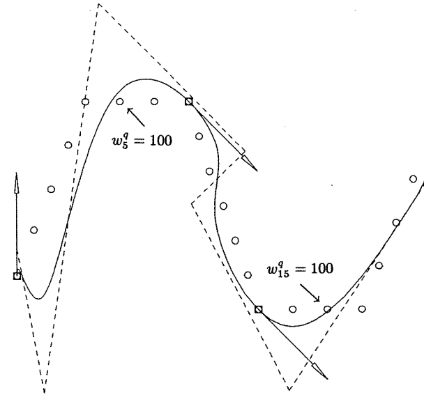
Figure 9.41. The curve from Figure 9.40, with weights w_5^q = w_{15}^q = 100 .
