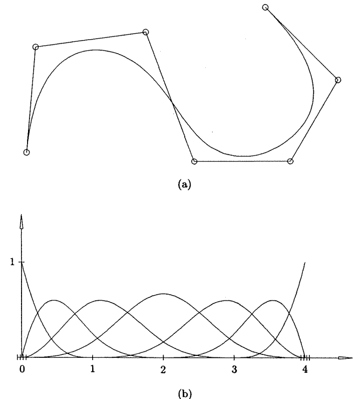
Figure 5.18. A cubic curve. (a) The curve and its control polygon; (b) basis functions defined over \{0, 0, 0, 0, 1, 2, 3, 4, 4, 4, 4\} .
