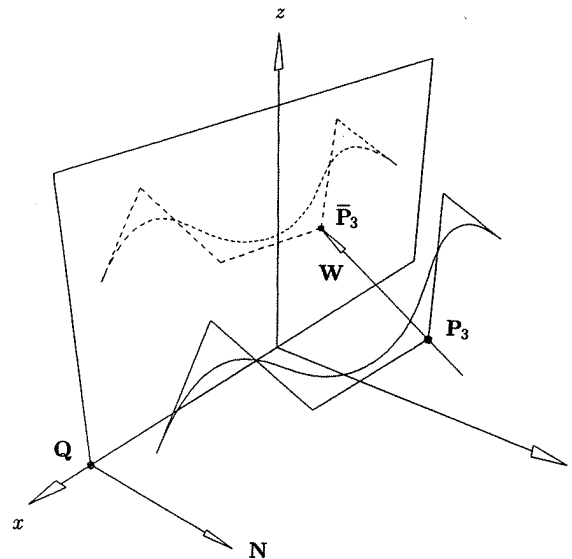
Figure 6.5. Parallel projection of NURBS curves.
