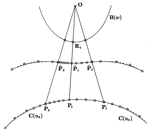
Figure 11.28. Curve bending.
