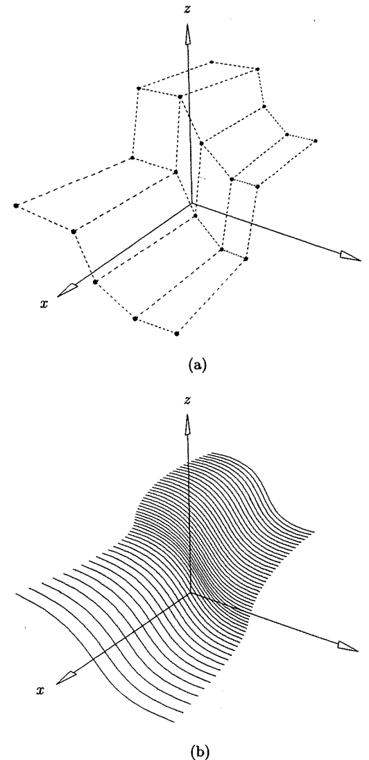
Figure 5.20. A (cubic \times quadratic) surface to be decomposed. (a) The control net; (b) the surface defined over U = \{0, 0, 0, 0, \frac{3}{5}, 1, 1, 1, 1\} and V = \{0, 0, 0, \frac{2}{5}, 1, 1, 1\} .
