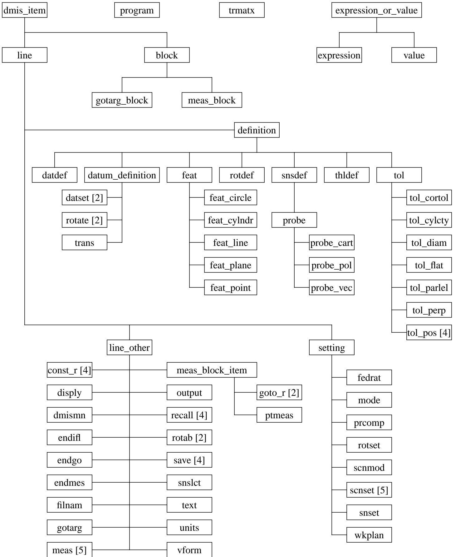
DMIS EXPRESS Schema Type Hierarchy a number in brackets indicates additional subtypes
