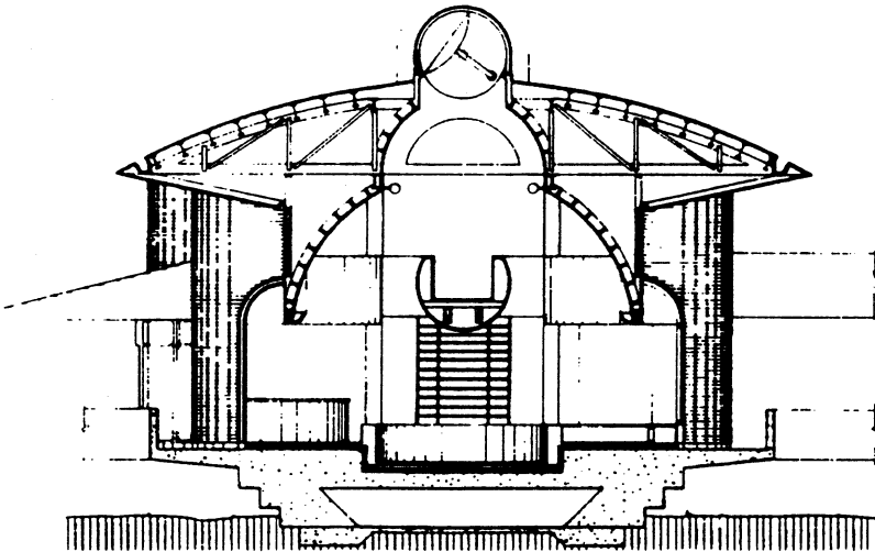
Cross section of energy self-sufficient home.
