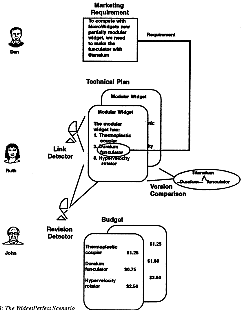
Figure 5: The WidgetPerfect Scenario
