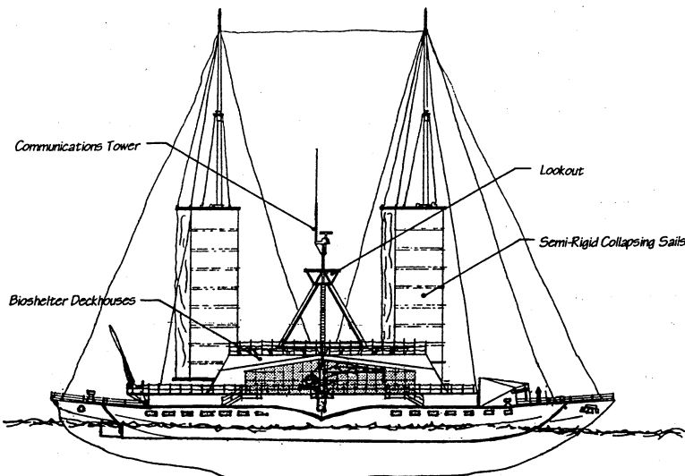
Trimaran Flagship with Semi-Rigid Sails
