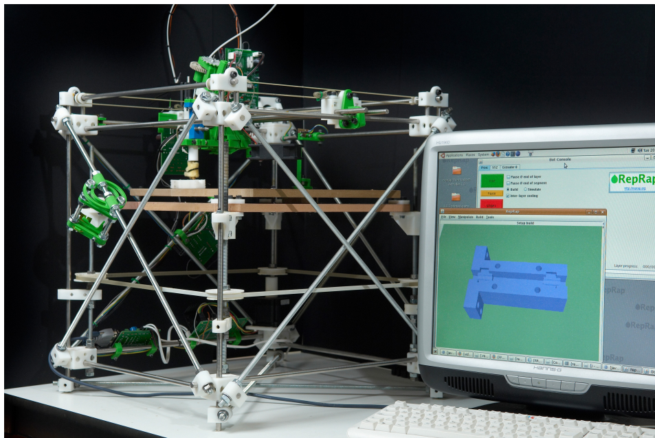
Figure 3. RepRap Version I “Darwin”. This is the first production RepRap machine. Its rapid prototyped parts (white, blue, and green) were made in a Stratasys Dimension commercial RP machine. The cube of the machine has side lengths of about 500 mm. This machine was built in May 2007.
