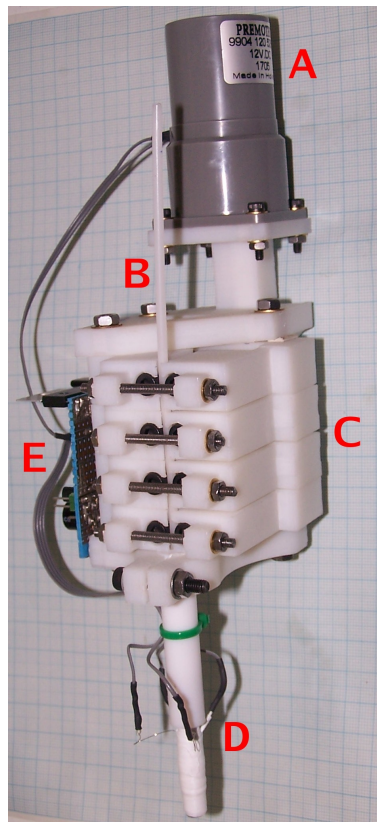
Figure 4. The first RepRap polymer transport mechanism.
