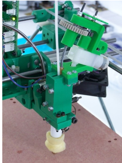
Figure 6. The last screw-driven RepRap polymer transport. All the green parts are rapid prototyped.
