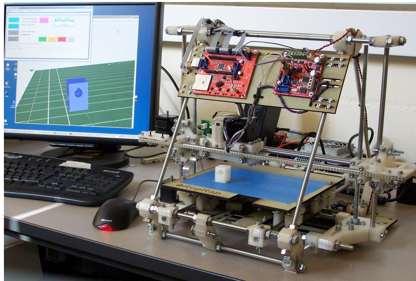
Figure 15. RepRap Version II “Mendel”. This is smaller, lighter and simpler than Version I, but it has a larger build volume.
