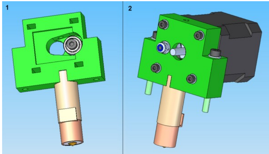
Figure 7. The current extruder transport mechanism (with melt chamber and nozzle at the bottom). 1: back view of the interior; 2: assembled.
