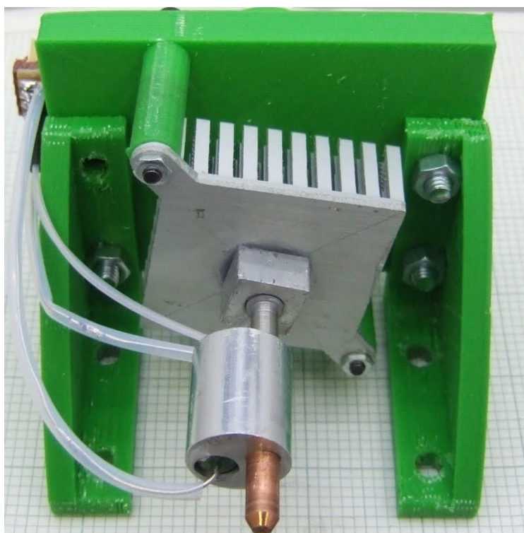
Figure 9. The stainless-steel heat-sink melt-chamber and nozzle.
