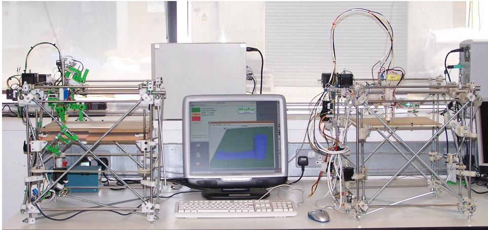
Figure 12. The first reproduced RepRap machine – parent (left) and child (right).
