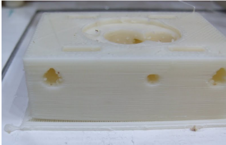
Figure 10. A RepRap extruder component made in a RepRap machine from ABS. Note the curling at the base.
