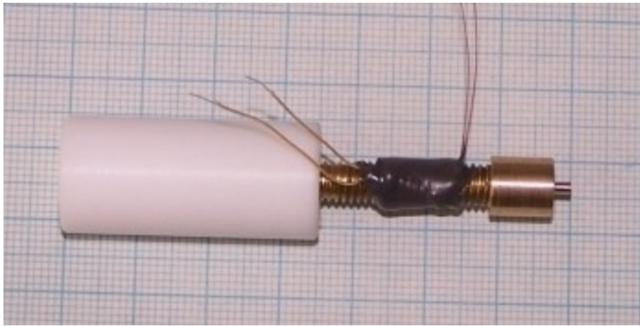
Figure 8. The first melt-chamber and nozzle design. The small squares are 1 mm.
