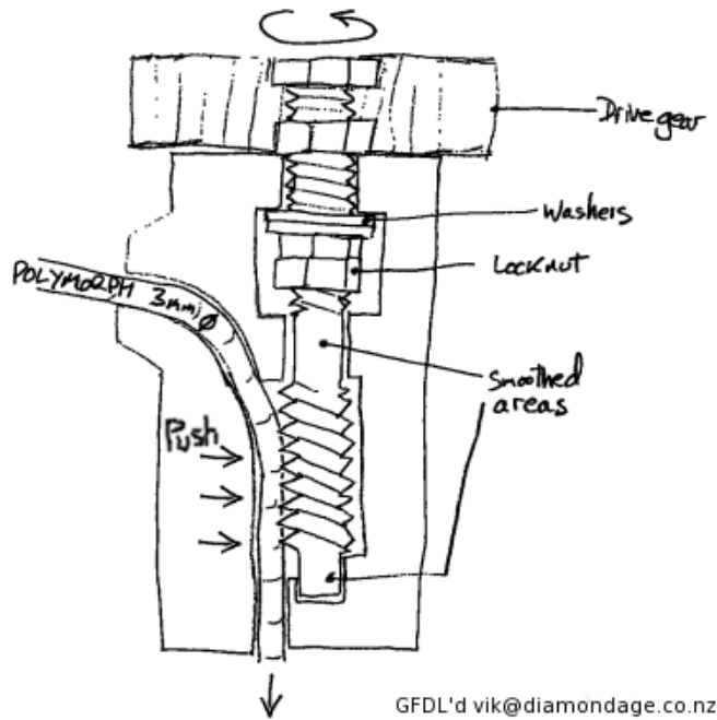
Figure 5. The screw-driven RepRap polymer transport (inventor's first sketch).
