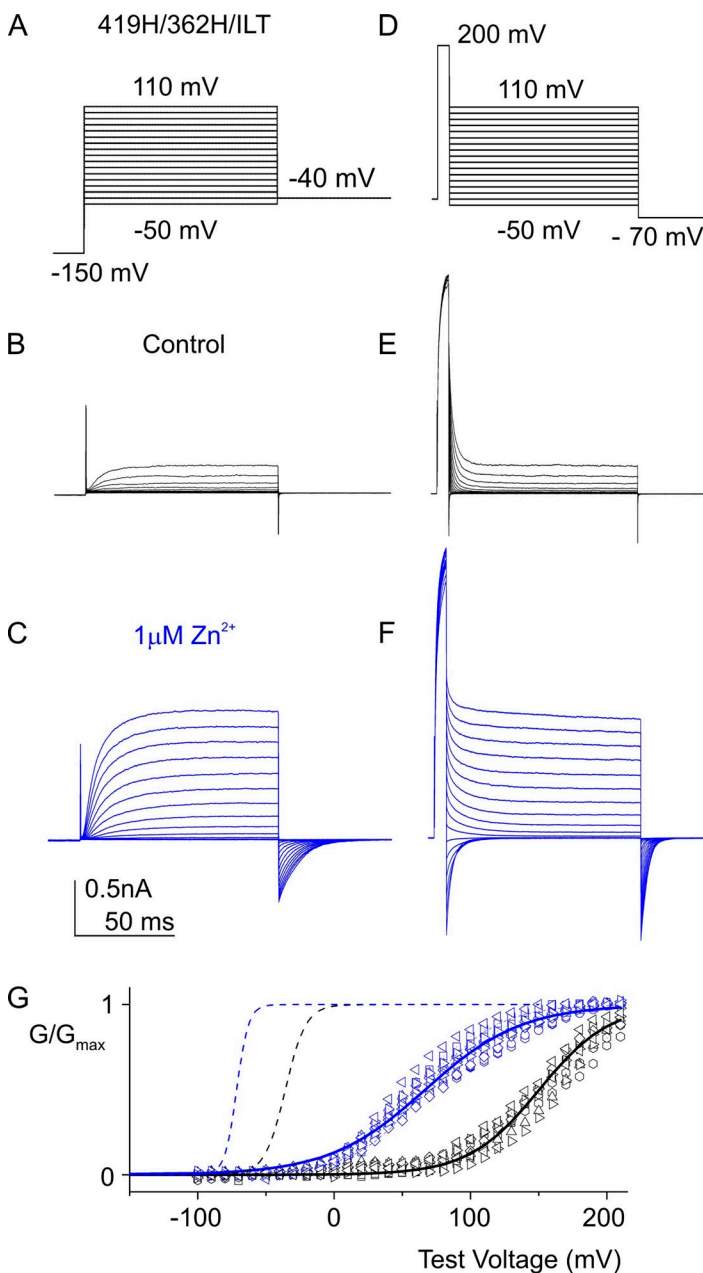
Figure 4. Zn^{2+} shifts the G-V relation of 419H/362H/ILT channels to negative voltages. Macroscopic currents from 419H/362H/ILT channels expressed in a HEK cell in either control external solution (black) or 1 \mu M Zn^{2+} (blue), and average steady-state conductance versus voltage relations determined from tail current measurements for a population of cells. (A) Voltage protocol illustrating 10-mV incrementing steps to voltages between -50 and +110 mV consecutively applied after a 150-ms prepulse to -150 mV. Holding voltage was -100 mV. (B) Representative macroscopic current records obtained in control solution using the protocol illustrated in A. (C) Macroscopic current traces recorded in the presence of 1 \mu M Zn^{2+} using the voltage protocol shown in A. (D) Voltage protocol illustrating 10-mV steps to voltages between -50 and +110 mV consecutively applied after a 12-ms prepulse voltage step to +200 mV to open the channels. (E) Representative macroscopic current records showing channel deactivation in control solution using the protocol illustrated in D. (F) Macroscopic current traces recorded in the presence of 1 \mu M Zn^{2+} using the voltage protocol shown in D. (G) Normalized steady-state channel conductance determined from tail current measurements after both activation (B and C) and deactivation (E and F), plotted as a function of membrane voltage. Each symbol type is from a different cell examined like the one illustrated in A–F. The G-V relation for each cell was fit with a single Boltzmann function and average values from these fits: V_{1/2} = 152.6 \pm 0.6 and z = 0.95 \pm 0.01 ; n = 13 for control; V_{1/2} = 66.52 \pm 0.8 and z = 0.72 \pm 0.08 ; n = 12 . Solid lines are single Boltzmann functions with mean values for V_{1/2} and z values. For reference, fits of single Boltzmann function to the G-V data for the non-ILT background (see Fig. 1) are plotted as dashed lines.
