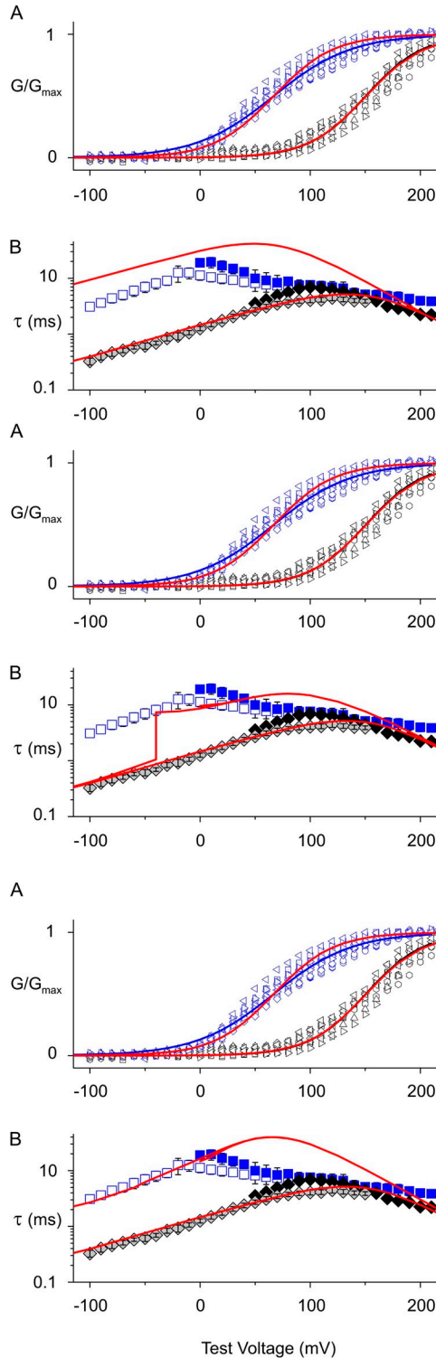
Figure 7. Kinetic models of 419H/362H/ILT channels that fail to describe gating of the channel in the absence or presence of Zn^{2+} . (Scheme 2) A three-state model in which Zn^{2+} binds to channels in the open state but not the pre-open state (O and A, respectively). (Scheme 3) A four-state model in which Zn^{2+} is allowed to bind to channels in both the open and pre-open states (O and A, respectively). (Scheme 4) A 10-state model with four independent Zn^{2+} binding sites, where Zn^{2+} can bind to channels in both the open and pre-open states (O and A, respectively). (A) Steady-state G-V relations in control (black) and 1 \mu M Zn^{2+} (blue) from Fig. 4 G. Model predictions are shown as red curves using the following rate constants. Scheme 2: k_o = 2.31 s^{-1} e^{(25.2V)} , k_c = 683 s^{-1} e^{(12.6V)} , k_b = 5.05 \times 10^{10} M^{-1}s^{-1} , and k_u = 2,200 s^{-1} ; Scheme 3: k_o = 2.31 s^{-1} e^{(25.2V)} , k_c = 683 s^{-1} e^{(12.6V)} , k_b = 7.5 \times 10^6 M^{-1}s^{-1} , k_u = 100 s^{-1} , and c = 100 ; Scheme 4: k_o = 2.31 s^{-1} e^{(25.2V)} , k_c = 683 s^{-1} e^{(12.6V)} , k_b = 8 \times 10^6 M^{-1}s^{-1} , k_u = 163 s^{-1} , and c = 30 . (B) Mean time constants ( \tau ) from the single-exponential fits to channel activation (filled symbols) and deactivation (open symbols), plotted as a function of the voltage in either control (black) or 1 \mu M Zn^{2+} (blue) from Fig. 5 G. Red lines represent time constants of the best fit of single-exponential functions to the simulated current relaxations using the scheme shown to the left and the rate constants given in A. Refer to Materials and methods for further description of these models.
