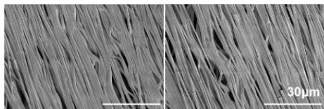
Figure S1 The SEM pictures of PLLA fiber under different concentration, receiving distance and rotate speed.
