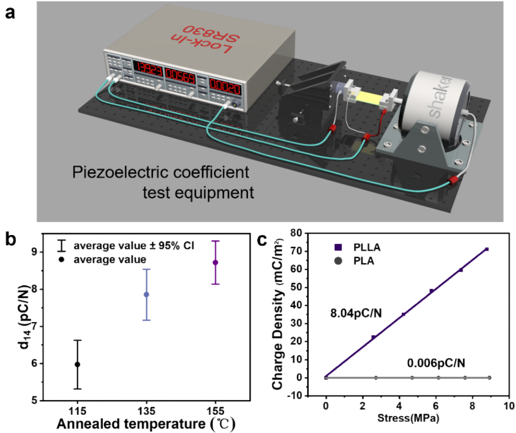
Figure S3 Measurement of piezoelectric coefficient. a, Schematic diagram of the measuring device for d_{14} piezoelectric coefficient. b, d_{14} of PLLA fiber under different annealing temperature. c, Output charge as a function of applied stress for the PLLA films of PLLA film and PLA film.
