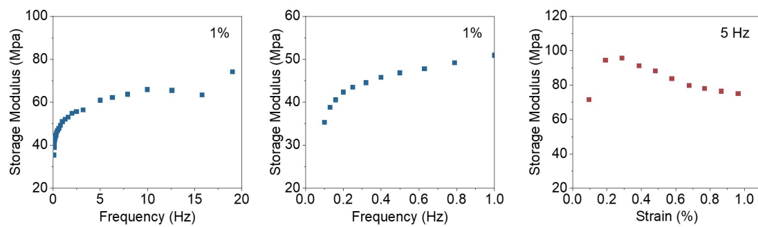
Figure S16 DMA test of unfolded ND-SENS film.
