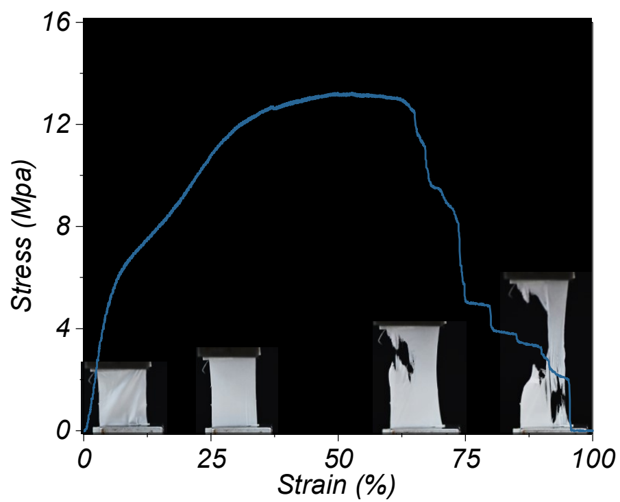
Figure S15 Stress-strain curve of unfolded ND-SENS film.
