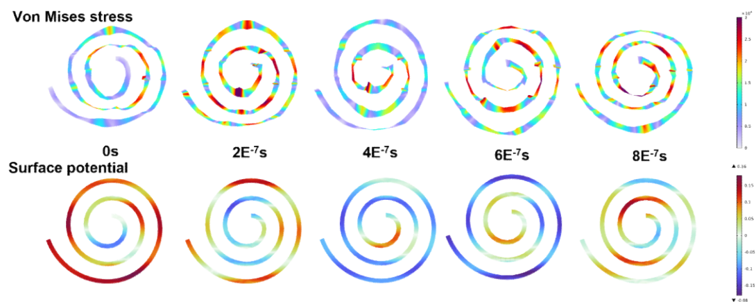
Figure S4 COMSOL simulation results of Von Mises stress and surface potential of PLLA film under ultrasound stimulation.
