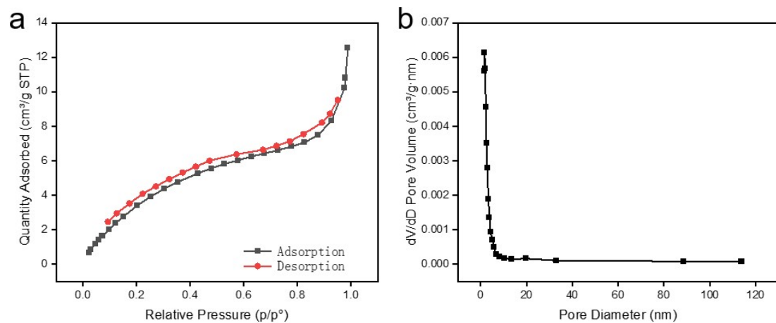
Figure S12. a) Isothermal adsorption curve of PLLA. b) BJH adsorption dV/dD pore volume of PLLA.
