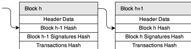
Figure 1: Block chain
