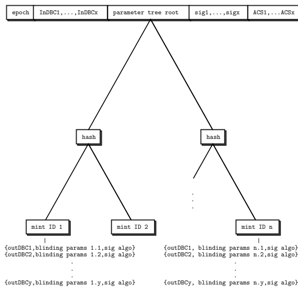
Figure 1: Transaction format (global set).
