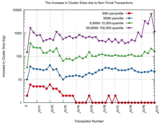
Figure 5. A plot of the q -th q -quantiles for q = 100, 1000, 10000, 100000 of the distributions of the increases in cluster size due to merging for every 250 000 transactions. The increases are heavily concentrated around median values of one. For the past 30 million transactions, the 99th percentiles are also at one.
