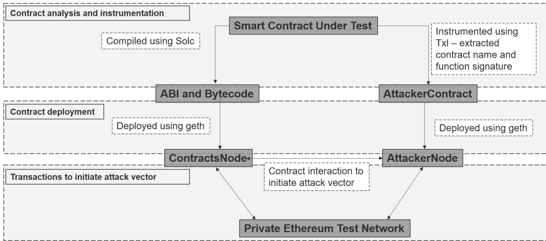
Fig. 3. Proposed Framework
