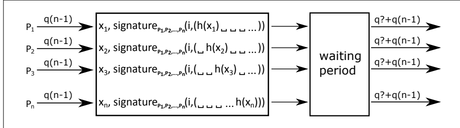
Fig. 2. Stateful contract for amortized multiparty fair SFE with penalties.
