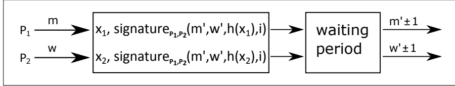
Fig. 3. Off-chain 2-party lottery.
