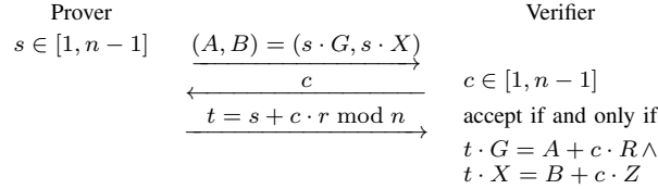
Figure 2: Chaum-Pedersen protocol [10]: a zero-knowledge proof technique to prove the statement that (G, X, R, Z) = (G, x \cdot G, r \cdot G, x \cdot r \cdot G) is a DDH tuple.
