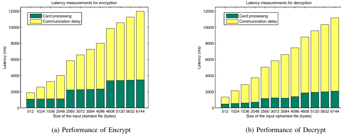
Figure 4: Performance evaluation based on a proof-of-concept implementation using a resource-constrained Java card (5 MHz processor). The same implementation should work several hundred times faster on a high-performance Tamper Resistant Module such as IBM Storage Manager HSM (2 GHz processor) [41].
