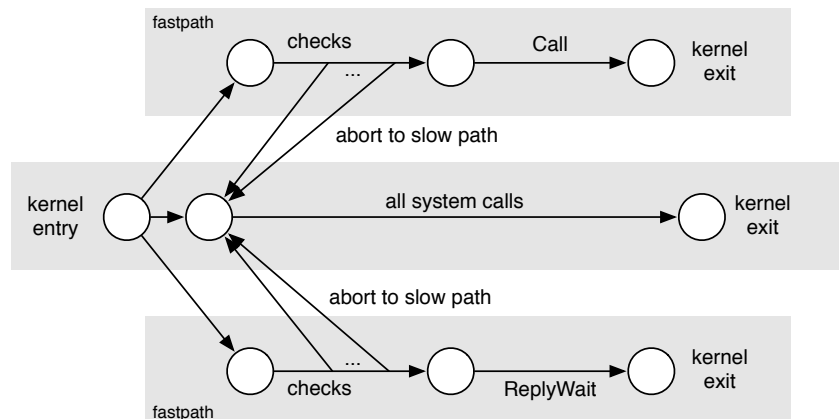
Fig. 11. Fastpath control flow.
