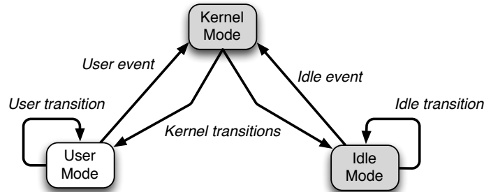
Fig. 10. Types of transitions.
