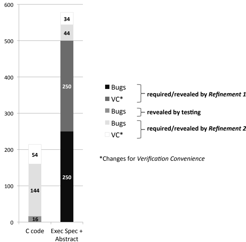
Fig. 20. Number of changes on the codes and models required by the verification.
