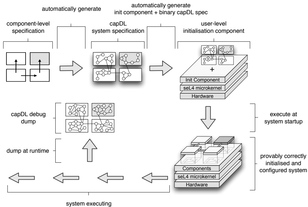
Fig. 15. Using capDL for correct system initialisation.
