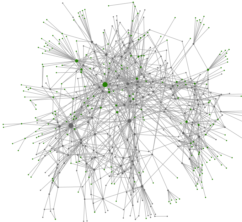
Fig. 1. Call graph of the seL4 microkernel. Vertices represent functions, and edges invocations.
