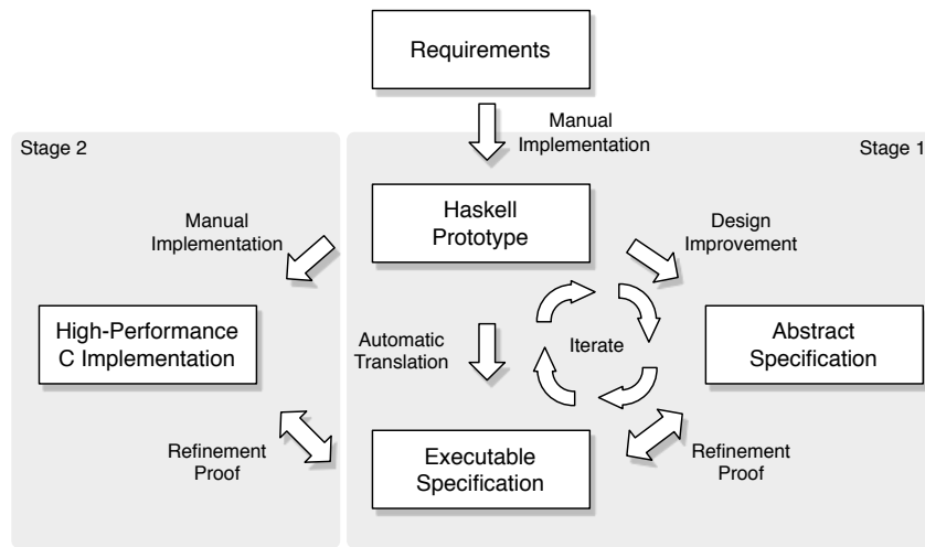
Fig. 2. The seL4 design process.
