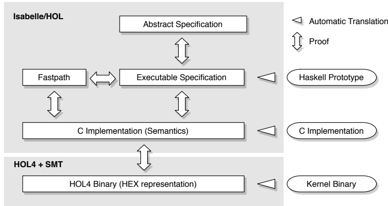
Fig. 9. Functional correctness proofs.
