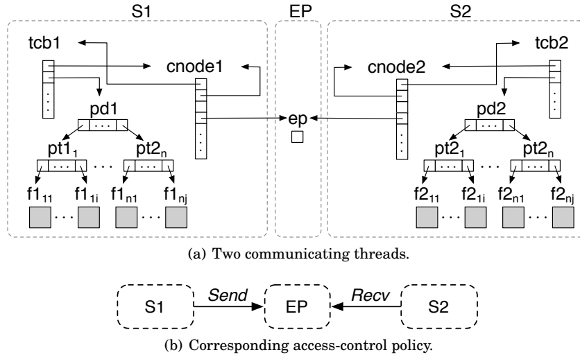
Fig. 13. System objects and corresponding access-control policy.
