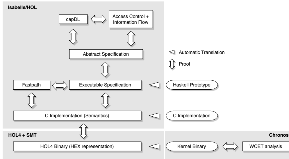
Fig. 3. The proof layers in the verification of seL4
