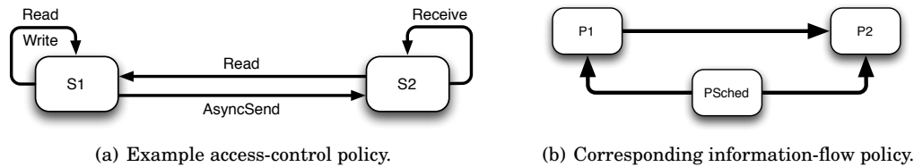
Fig. 14. Access control policy and corresponding information-flow policy.
