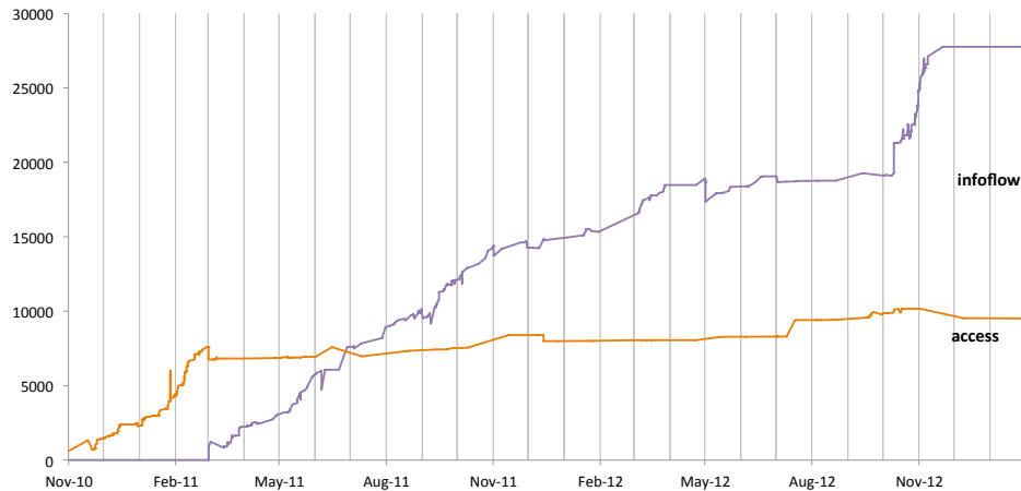
Fig. 18. Size of security proofs—detailed.
