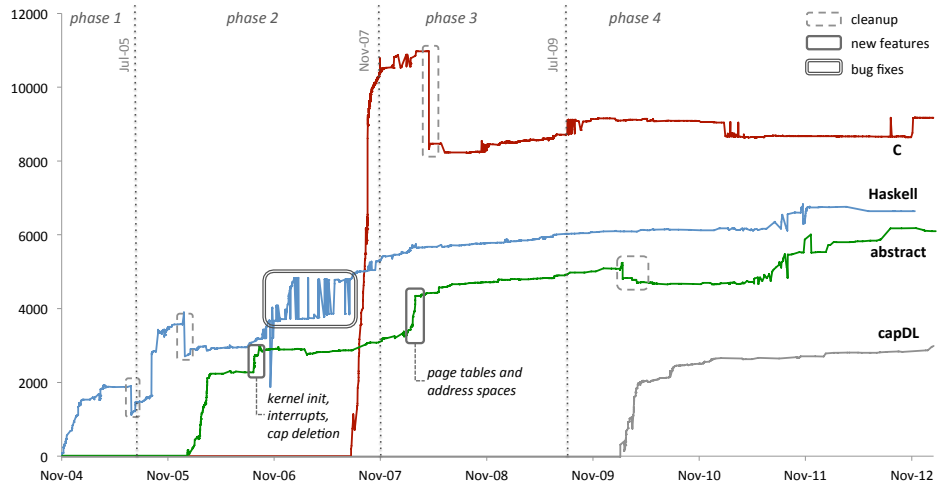
(a) Size of code/spec artefacts (X: time; Y: SLOC)
