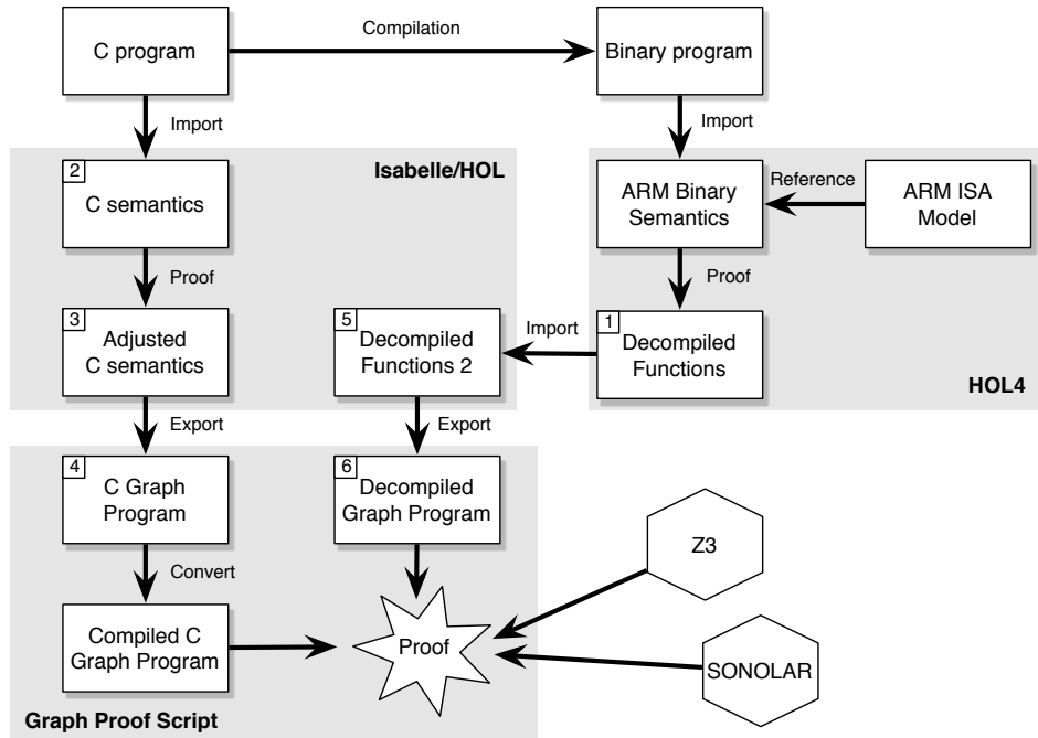
Fig. 12. Binary verification overview for seL4.
