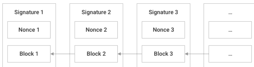
Figure 1: A validator votes for blocks with one-time signatures.
